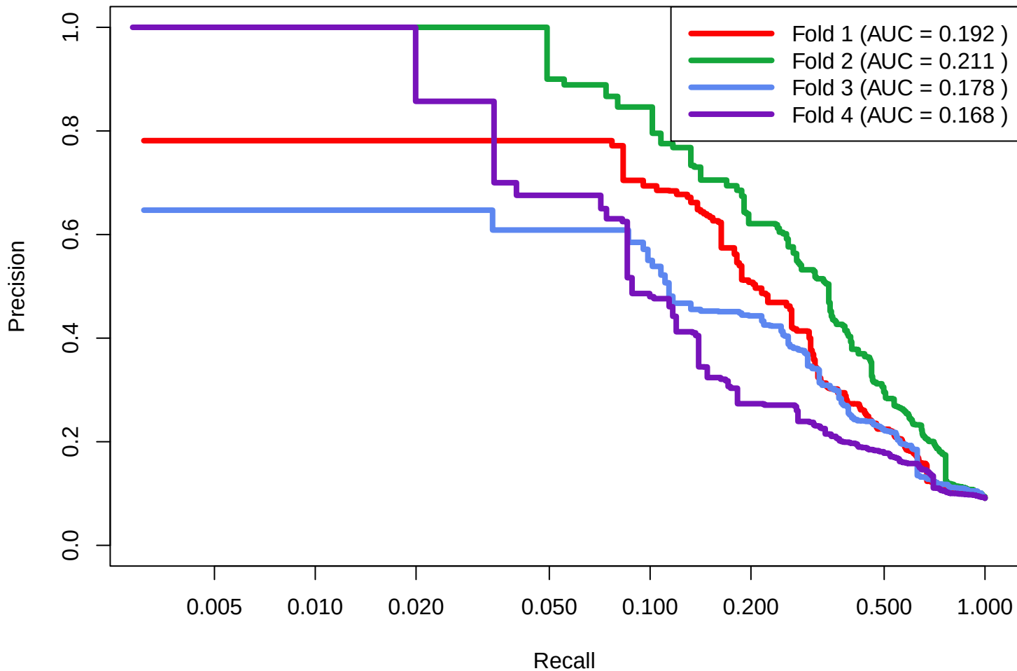
SPELL All Datasets: 430x200x1 Validation
